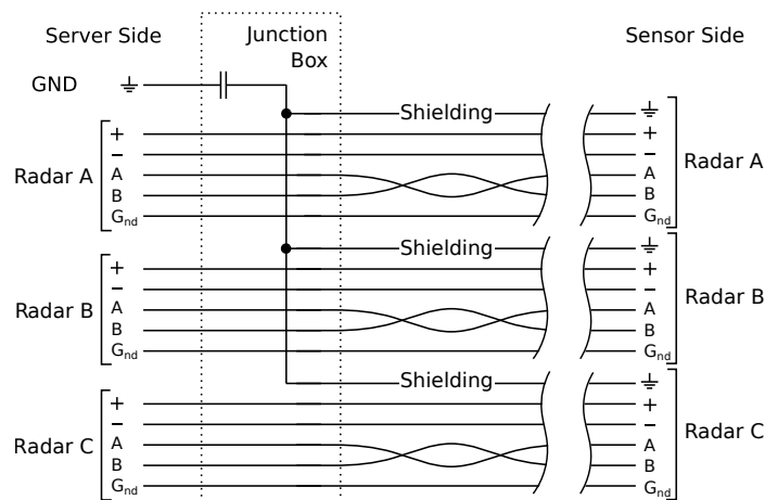
Figure 2.3: The three cable connection diagram between the WaveGuide processing unit and radars when the radars are powered from the processing unit.
