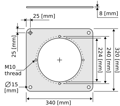
Figure 1.9: Optional mounting plate for an non Ex. certified WaveGuide Radar (product no. WG-MP-SS).
