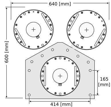
Figure 1.6: Top view of a point array installation mounted on a standard mounting frame (product no. WG-MD-SS).
