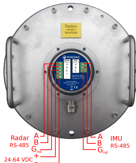
Figure 2.1: Terminal compartment and connections.
